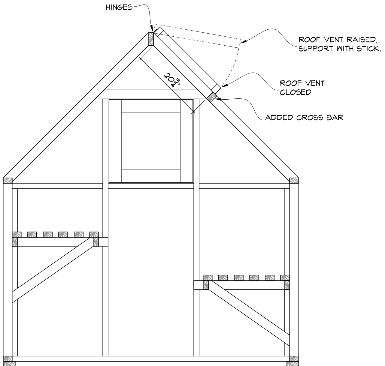
SECTION VIEW
